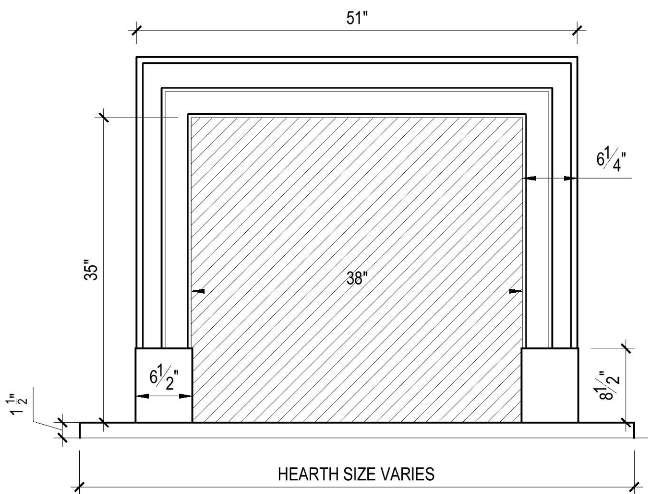
FRONT
