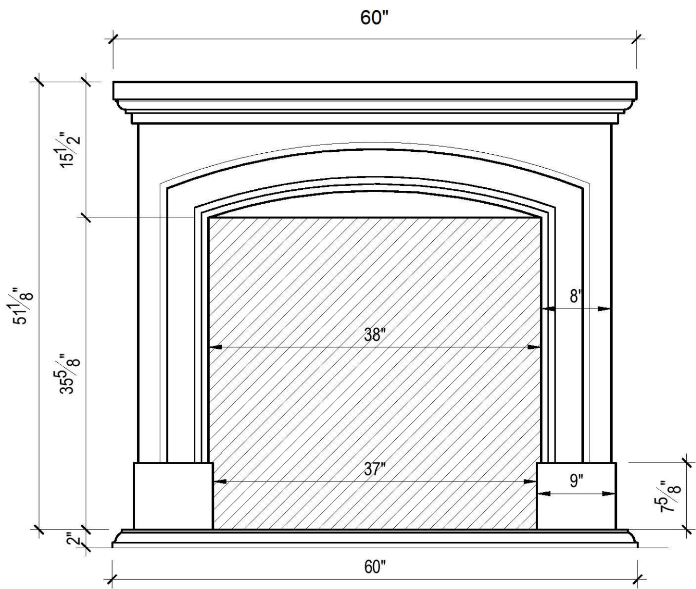
FRONT
